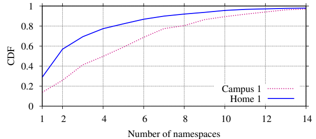
Figure 13: Number of namespaces per device.
