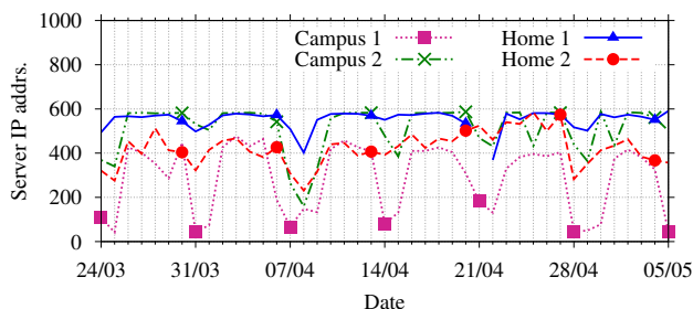
Figure 5: Number of contacted storage servers.
