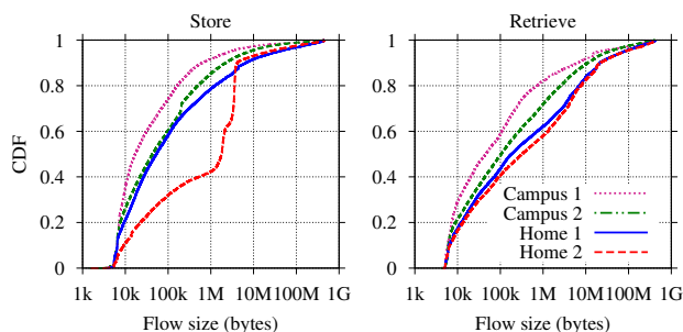
Figure 7: Distribution of TCP flow sizes of file storage for the Dropbox client.
