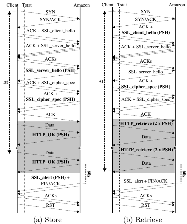
Figure 19: Typical flows in storage operations.
