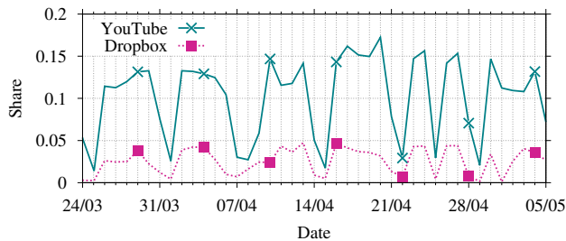
Figure 3: YouTube and Dropbox in Campus 2 .
